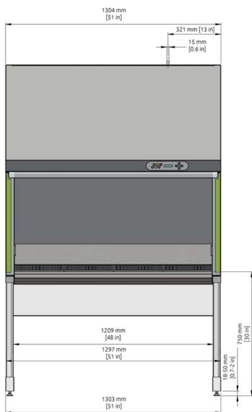
Closed Front
